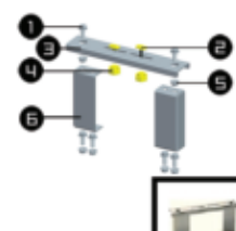
Cabinet top stand
