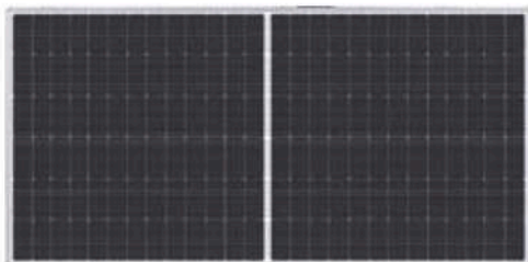
N-Type, HALF-CELL, Mono N-Type 182 mm, 600-625W IP68
