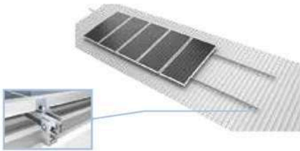
METAROOF-MK KILPLOCK WITHOUT RAIL SYSTEM
