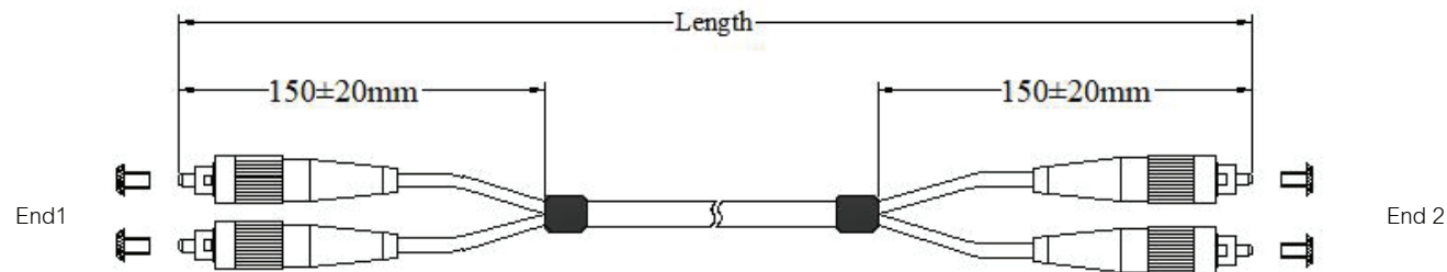
FC 2.0mm&3.0mm duplex patchcord
