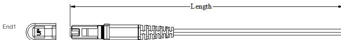
MTRJ 2.0mm duplex patchcord
