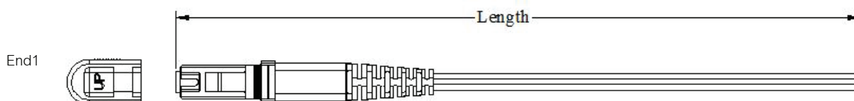
MTRJ 0.9mm duplex pigtail
